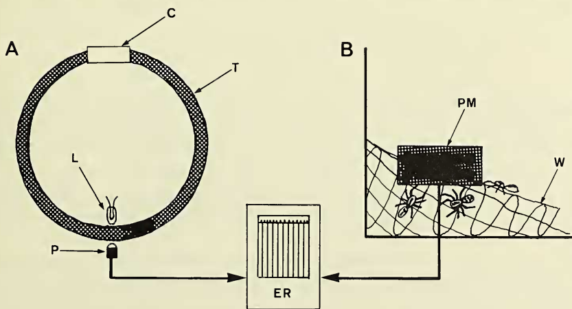
Fig. 2—Photoelectric recording methods. A: Apparatus to measure activity of isolated Mallos gregalis . Tygon tubing (T), held end-to-end by a coupling tube (C) contained the animals. Movement of spiders between the phototransistor (P) and biasing lamp (L) was recorded on one channel of an event recorder (ER). Colony activity (B) used a photocell matrix (PM). Movement of spiders on the web (W) was recorded as in A.
